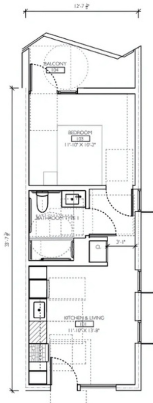
03 UNIT TYPE 3 / 1-BEDROOM SCALE 1/4" = 1'-0"
