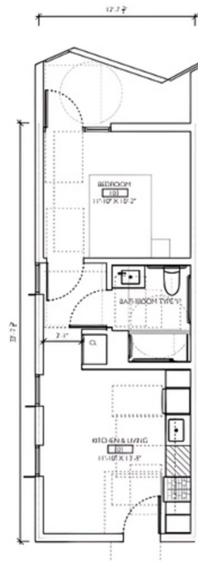
UNIT TYPE 3 / 1-BEDROOM
