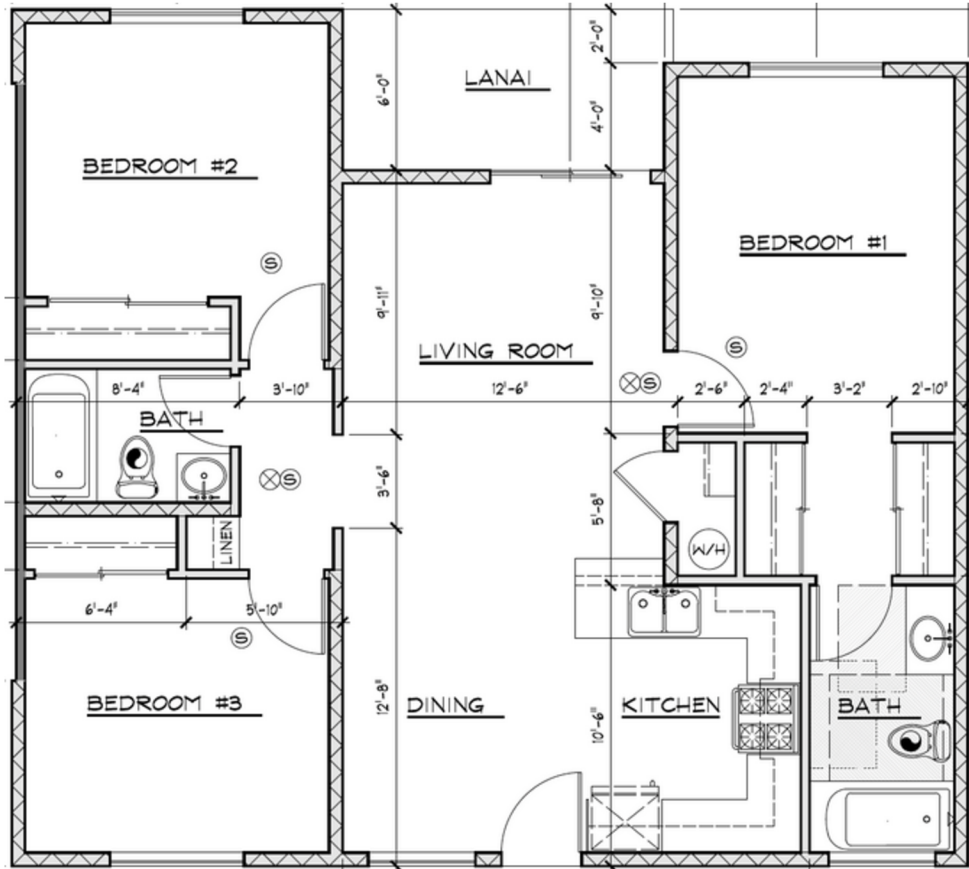
Floor Plan - Unit Type 3
