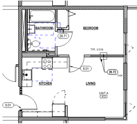
UNIT TYPE A (1-BEDROOM)- NEW CONSTRUCTION
